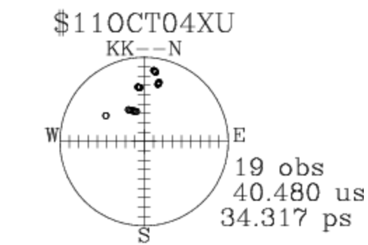
Worst STN: sky coverage and UT1 formal error in \mu s
