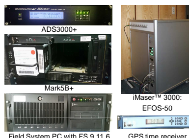
Newly installed data acquisition systems for VLBI
