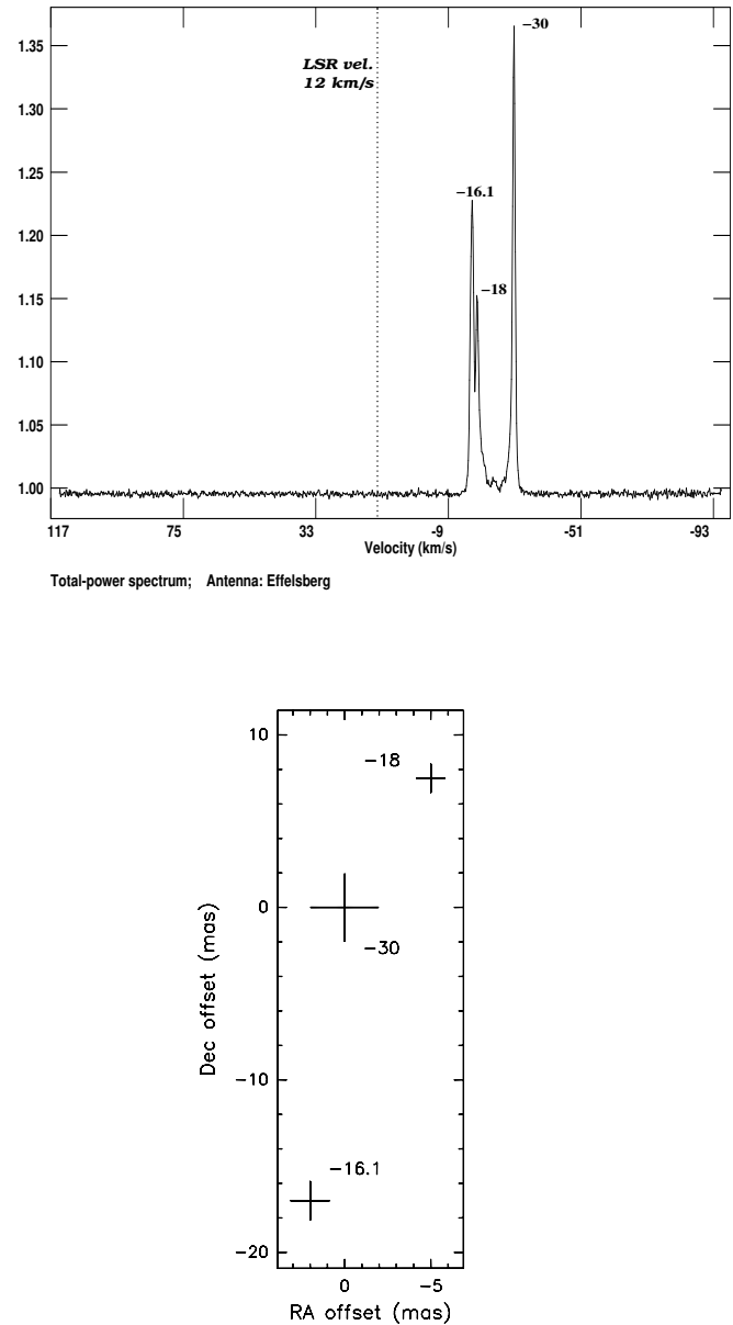
Fig. 5. Upper: Effelsberg total power spectrum for GGD12-15. The vertical dotted line indicates the systemic LSR velocity. The labels indicate the velocities in [km/s] of the most prominent features, for which we have made maps. Lower: Distribution of H 2 O maser spots corresponding to the dominant emission features in the total power spectrum. The channel with the highest emission (vel. -30 km s -1 ) was used as reference in the astrometric analysis. The labels in the plot indicate the velocities corresponding to each spot, in [km/s]; the size of the crosses is proportional to the square root of the peak flux in the maps.
