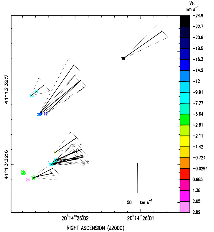
Fig. 2. Map of H 2 O maser spots and measured proper motions, measured from global VLBI multiepoch observations.
