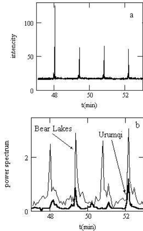
Fig. 1. a) Recording of echo intensity of “Raduga-9”; time resolution dt=0.017 s; estimated period of rotation is 83 s; b) Dependence of spectral maximum on time (cross-spectrums for “Raduga-9” on Evpatoria-Bear Lakes and Evpatoria-Urumqi baselines), time resolution dt=4.26 s, real period of rotation is 166 s.
