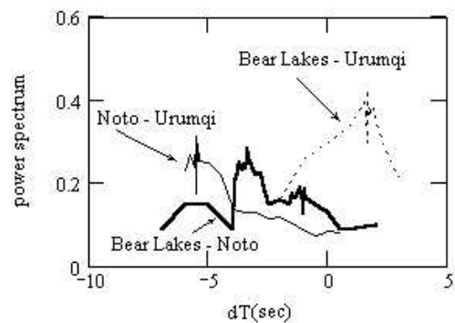
Fig. 2. Time dependence of cross-spectrum maximums of “Cosmos-1366” at baselines Bear Lakes – Noto, Bear Lakes – Urumqi and Noto – Urumqi (25 July, 2003).
