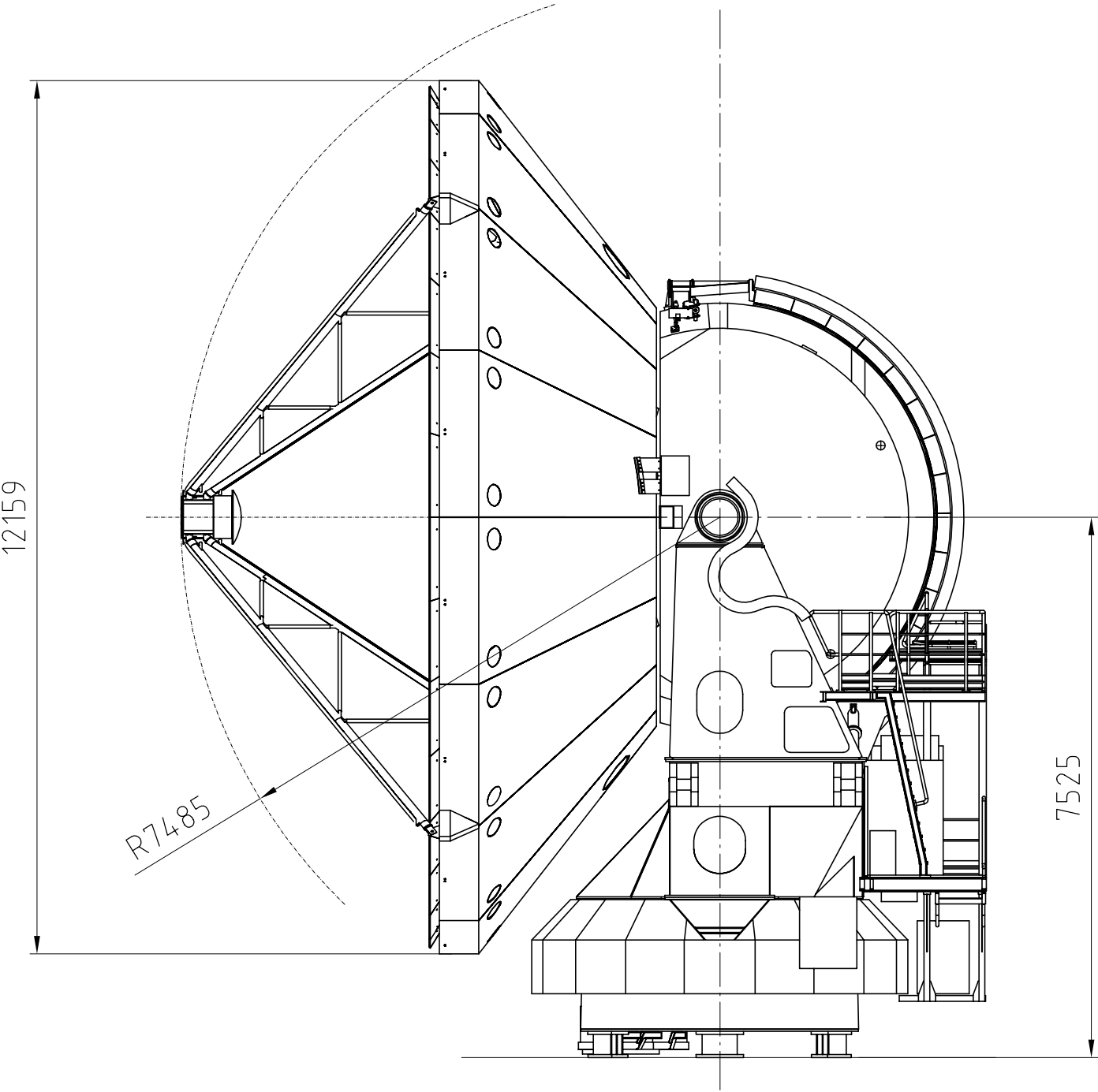
ANTENNA AT 0°
