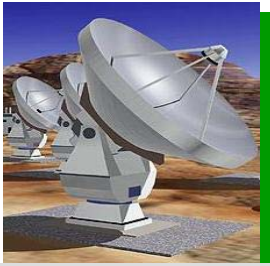
ALMA Project
