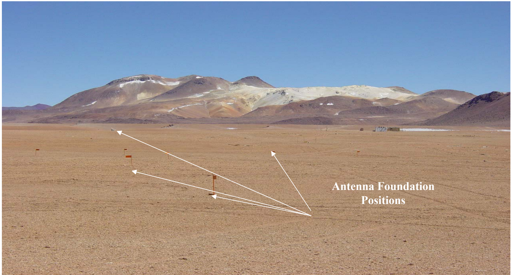
ALMA Project
