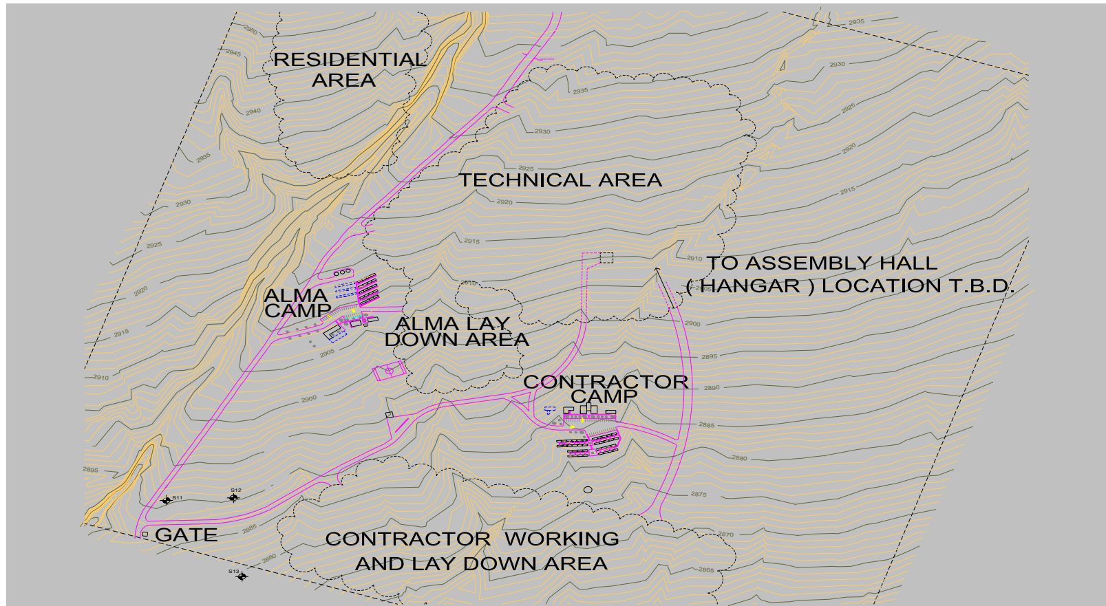
ALMA Project
