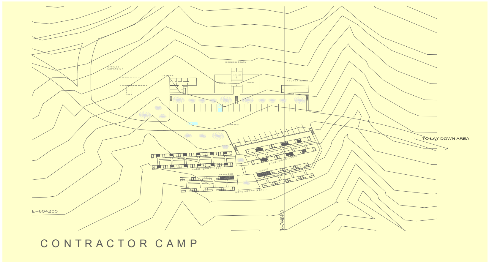
ALMA Project
