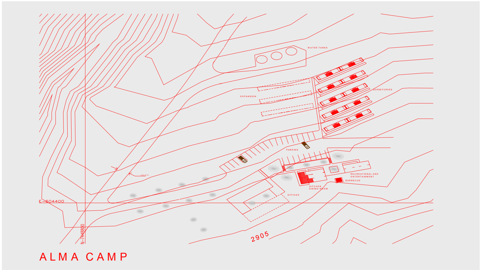
ALMA Project
