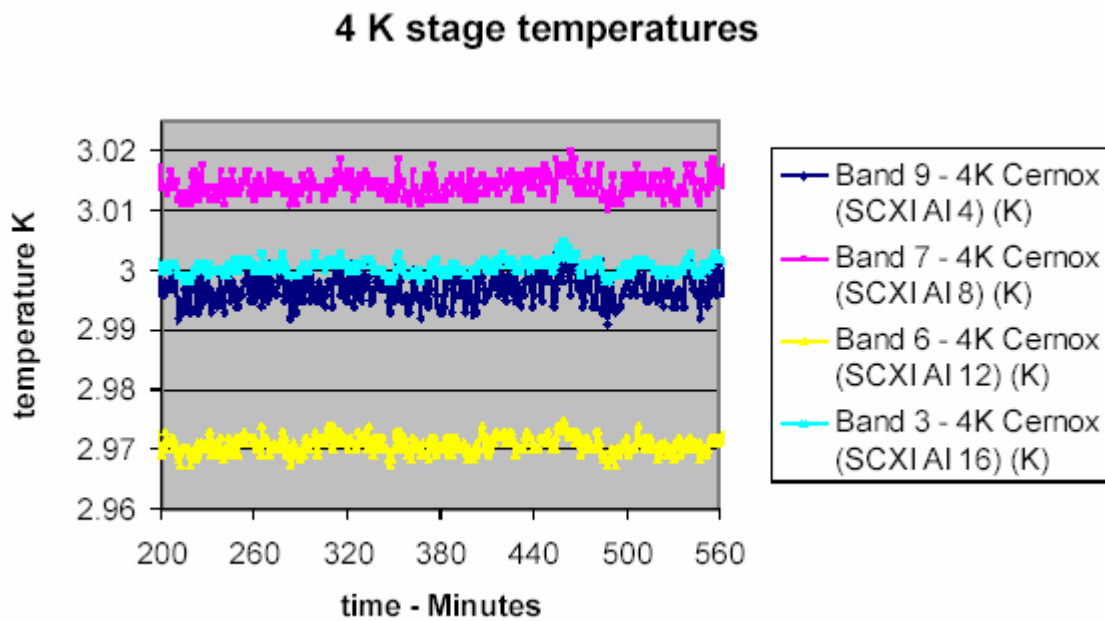
Figure 18. Temperature of the 4 K cryostat stage vs. time.
