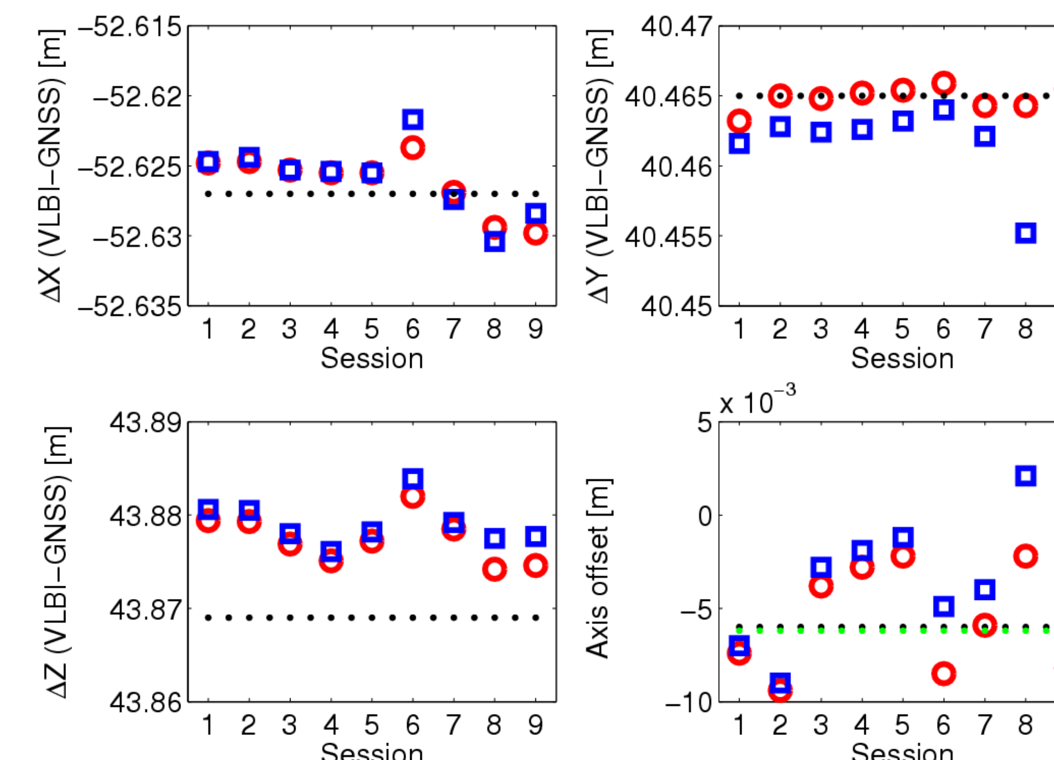
Fig. 6 Results for local tie vector and axis offset [4].
